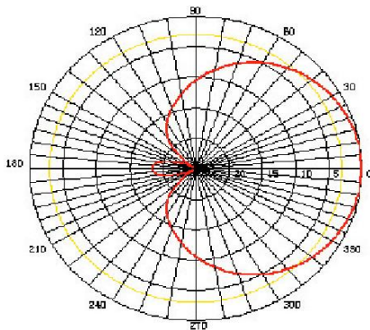
H Plane - Azimuth
