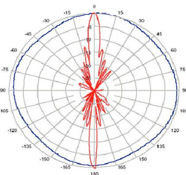
13 dBi Antenna
