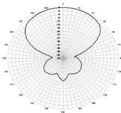
90-9 Horizontal Plane
