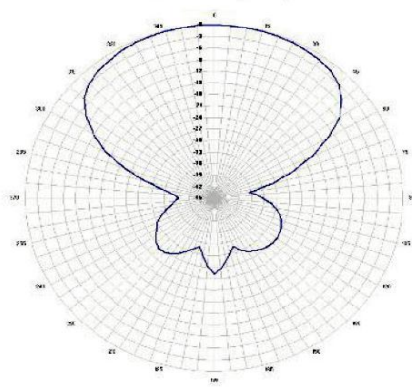
90-17 Horizontal Plane
