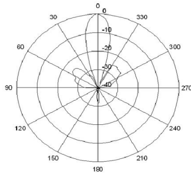
AWSPA5818 E Plane
