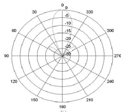
AWSPA5818 H Plane
